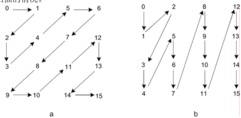
图 8-8—4x4块扫描 (a)Z型扫描(b)域扫描 (资料性)
